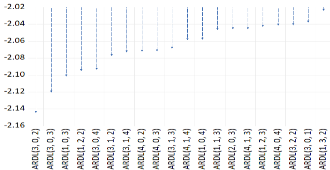
Akaike Information Criteria (top 20 models)
