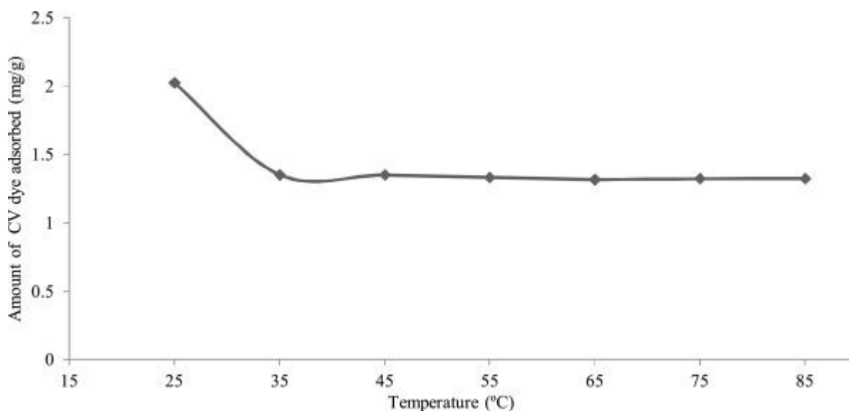
Figure 6: Influence of temperature on crystal violet adsorption (WCH: 0.25 g/50 mL; initial dye concentration: 12.2394 mg/L; particle size: 0.15–3.0 mm).
